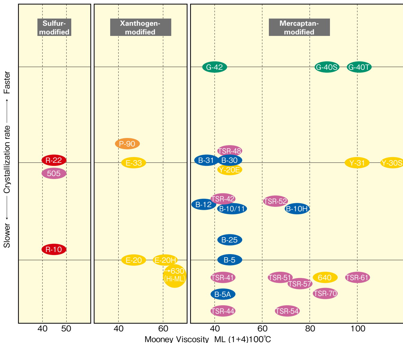
Figure-2 Skyprene Grades and Characteristics
