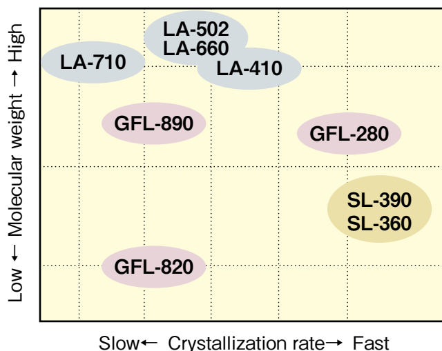
Figure-6 Characteristics and Relationship of Latex Grades
