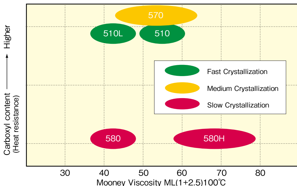
Figure-5 Characteristics and Relationship of Heat resistant Grades
