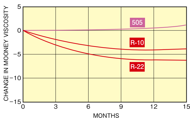
Figure-3 Stock stability of R-10, R-22 and 505, change in mooney viscosity at room temperature
