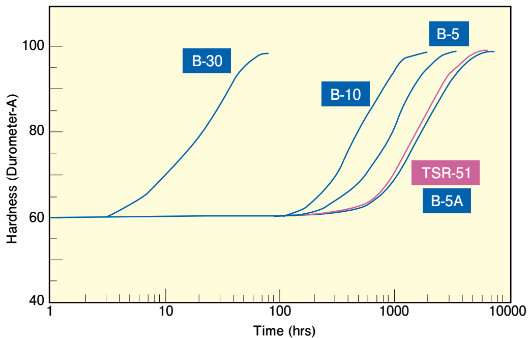
Figure-1 Change in hardness of Skyprene at -10^{\circ}\text{C} (standard formulation, cured 20 minutes at 150^{\circ}\text{C} )
